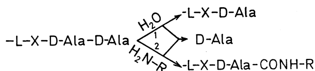
FIGURE 2. Reactions catalysed by the PSEs on L-X-D-Ala-D-Ala terminated peptides. 1, DD-carboxypeptidase activity; 2, transpeptidase activity. \text{H}_2\text{N-R} = \text{Gly, D-Ala} or a more complex amino compound.
